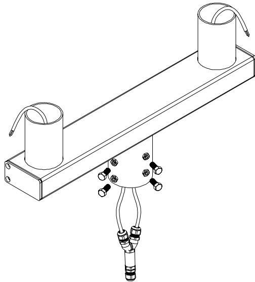
Double head pole mount adapter, 180°, On-Off, for 76mm spigot diameter Ordering Code : AUN-MOT-0070-XX
