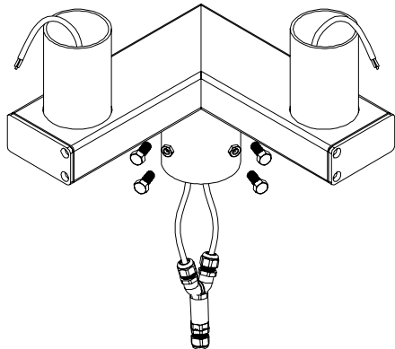
Double head pole mount adapter, 90°, On-Off, for 76mm spigot diameter Ordering Code : AUN-MOT-0069-XX
