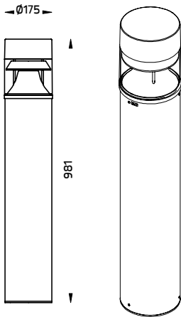
Double FUJI Flat – Bollard
