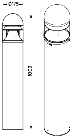
Double FUJI Round – Bollard
