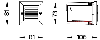
DOT Square Grill
