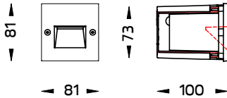
DOT Square Ramp
