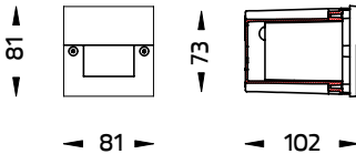
DOT Square Eyelid DOT Opal Square Eyelid
