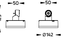
Round base for Ground mount [1-10V or Dali] [pre-assembled from factory] Ordering Code/รหัสสั่งซื้อ : AUN-MOT-0022-XX
