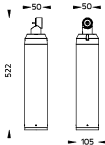
Short Pole. [On,Off] [pre-assembled from factory] Ordering Code/รหัสสั่งซื้อ : AUN-POL-0043-XX
