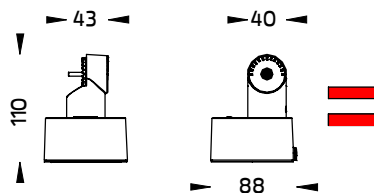
Round base for Ground mount. [On/Off] (pre-assembled from factory) Ordering Code/รหัสสั่งซื้อ : AUN-MOT-0052-XX
