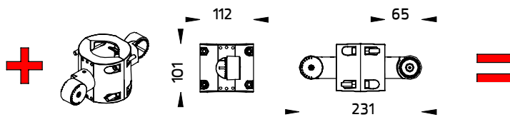
Pole Clamp Double Side Diameter 60-76mm. [On/Off] [pre-assembled from factory] Ordering Code/รหัสสั่งซื้อ : AUN-CLP-0053-XX
