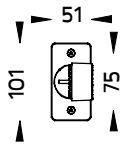
Pole mount adaptor for pole dia 60mm. [On/Off] (pre-assembled from factory) Ordering Code/รหัสสั่งซื้อ : AUN-MOT-0055-XX
