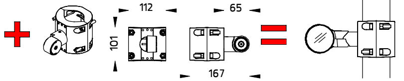
Pole Clamp Single Side Diameter 60-76mm. [On/Off] [pre-assembled from factory] Ordering Code/รหัสสั่งซื้อ : AUN-CLP-0052-XX
