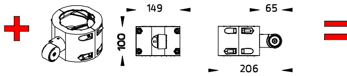
Pole Clamp Single Side Diameter 102-105mm. [On/Off] [pre-assembled from factory] Ordering Code/รหัสสั่งซื้อ : AUN-CLP-0054-XX
