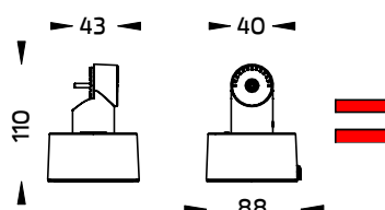
Round base for Ground mount. [On/Off] (pre-assembled from factory) Ordering Code/รหัสสั่งซื้อ : AUN-MOT-0052-XX
