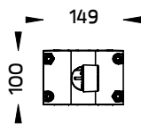
Pole Clamp Double Side Diameter 102-105mm. (On/Off) [pre-assembled from factory]
