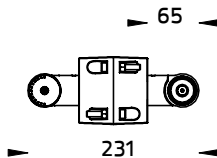
Pole Clamp Double Side Diameter 60-76mm. [On/Off] (pre-assembled from factory) Ordering Code/รหัสสั่งซื้อ : AUN-CLP-0053-XX
