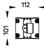
Pole Clamp Double Side Diameter 60-76mm. [On/Off] (pre-assembled from factory) Ordering Code/รหัสสั่งซื้อ : AUN-CLP-0053-XX
