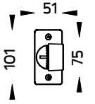
Pole mount adaptor for pole dia 102-105mm. [On/Off] [pre-assembled from factory]
