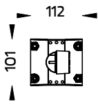
Pole Clamp Single Side Diameter 60-76mm. [On/Off] (pre-assembled from factory) Ordering Code/รหัสสั่งซื้อ : AUN-CLP-0052-XX
