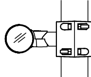
Pole Clamp Single Side Diameter 60-76mm. [On/Off] (pre-assembled from factory) Ordering Code/รหัสสั่งซื้อ : AUN-CLP-0052-XX
