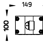
Pole Clamp Single Side Diameter 102-105mm. [On/Off] (pre-assembled from factory) Ordering Code/รหัสสั่งซื้อ : AUN-CLP-0054-XX
