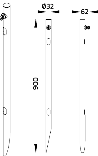
Earth spike, L 900mm, aluminum, single side luminaire mounting (pre-assembled from factory) Ordering Code/รหัสสั่งซื้อ : AUN-ESP-0006-XX
