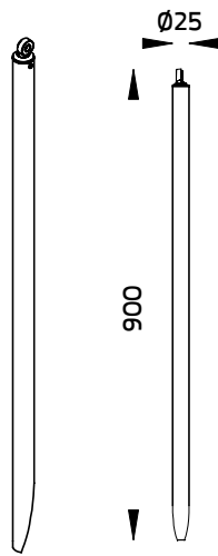
Earth Spike L 900mm, aluminum, (pre-assembled from factory) Ordering Code/รหัสสั่งซื้อ : AUN-ESP-0003-XX
