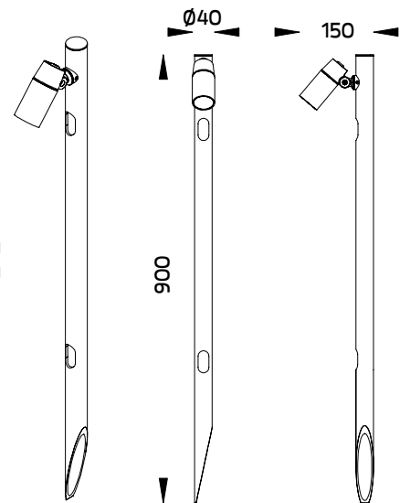
Earth spike, L 900mm, aluminum, single side luminaire mounting (pre-assembled from factory) Ordering Code/รหัสสั่งซื้อ : AUN-ESP-0006-XX
