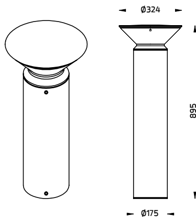
AGAR Opal - Direct Light Bollard
