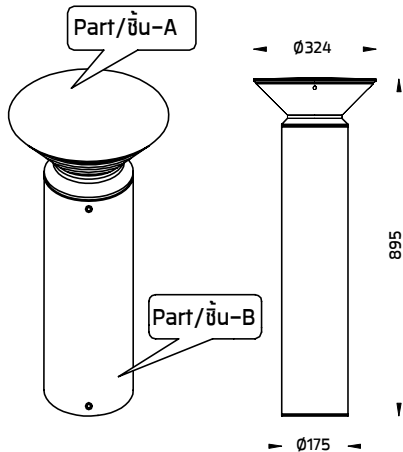
AGAR Prismatic - Indirect Light Bollard
