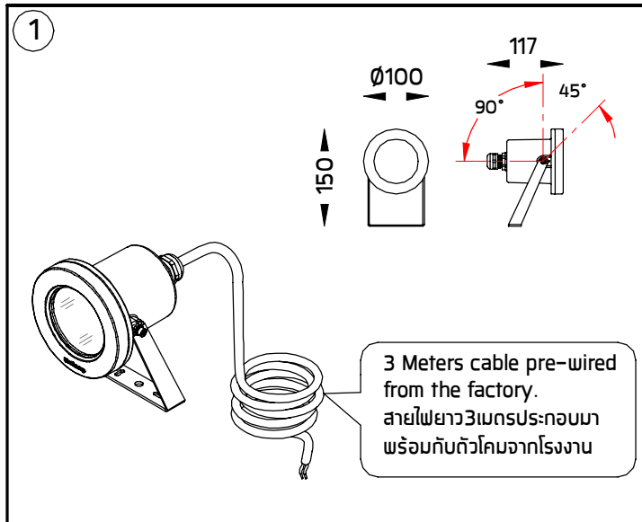
1 Light Emitting Diodes (LED) GU5.3
