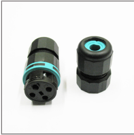
Ordering Code: 9-0903-00 IP68 Water Tight Connecting Device Cable Diameter 7 – 12mm.
