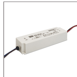
Ordering Code: 0486-0-9-000-00 LED Constant Voltage Driver 12Vdc 100W.
