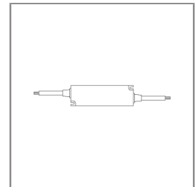
Ordering Code: AUN-DRG-0118-00 LED constant voltage driver, 24VDC, 30W
