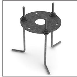
Ordering Code: AUN-ACB-0007-00 Anchor bolt kit
